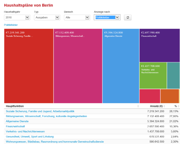
Figure 5 - Treemap
