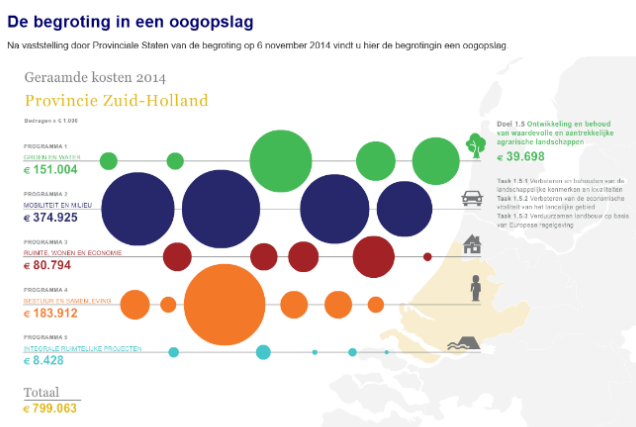
Figure 4 – Bubble chart
